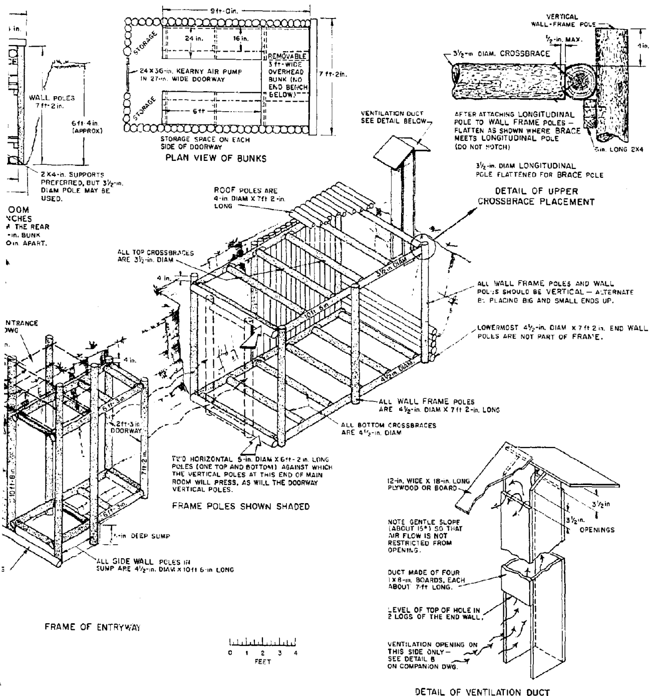
Fig. A-1.1. Small-Pole Shelter, Pictorial View.
